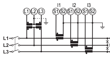
Fig. 10 Three-phase system without neutral (3-wire, 3P), unbalanced load, 3 CT and 2 VT/PT.
